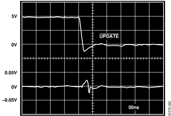
Figure 37. AD8114 Switching Transient (Glitch)
