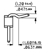
KINK DETAIL C
