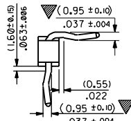
KINK DETAIL G
