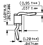
KINK DETAIL F
