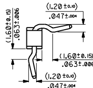
KINK DETAIL D
