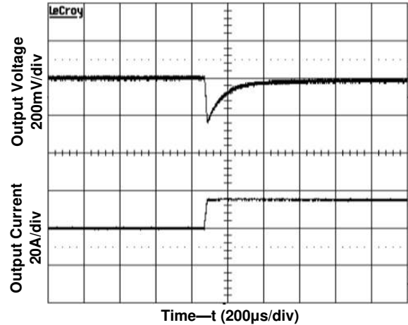
Figure 9. Transient Load Response Input voltage 12V, Output current 22.5A->33.7A, Slew rate 1A/µs
