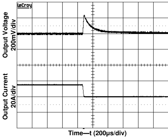
Figure 8. Transient Load Response Input voltage 12V, Output current 33.7A->22.5A, Slew rate 1A/µs
