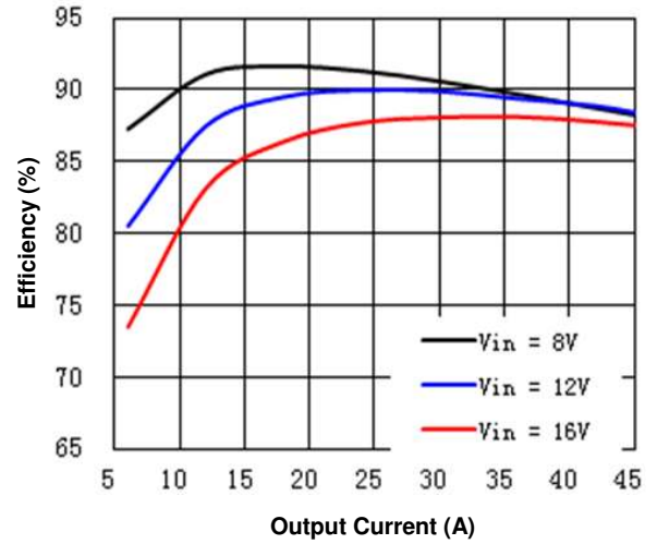
Figure 1(d). Efficiency vs. Load Current (25°C, 1.5V)
