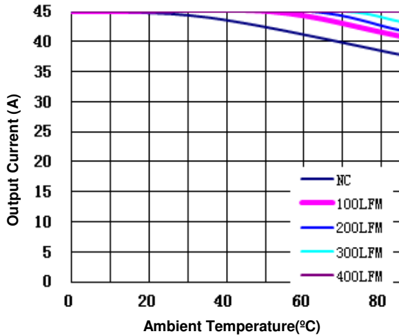
Figure 10(d). Current Derating Curve for 1.5V Output
