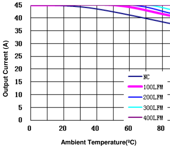
Figure 10(e). Current Derating Curve for 1.8V Output
