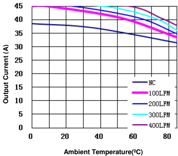
Figure 10(g). Current Derating Curve for 3.3V Output
