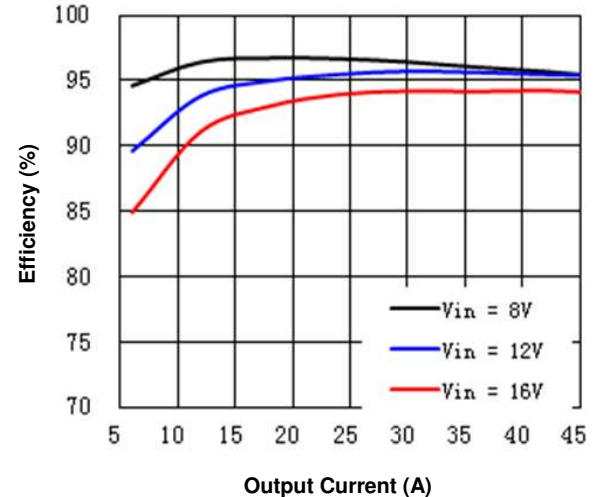
Figure 1(h). Efficiency vs. Load Current (25°C, 5V)
