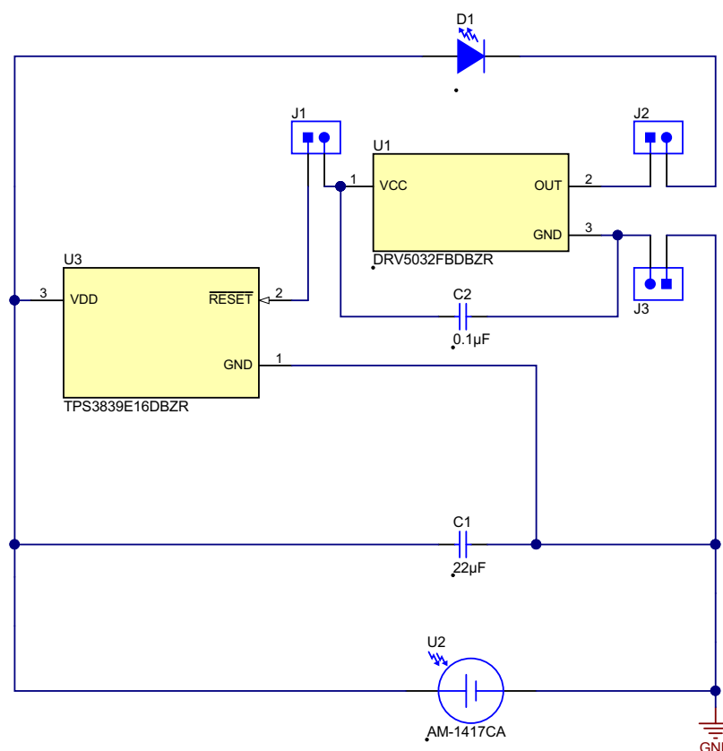
Figure 1. DRV5032-SOLAR-EVM Schematic
