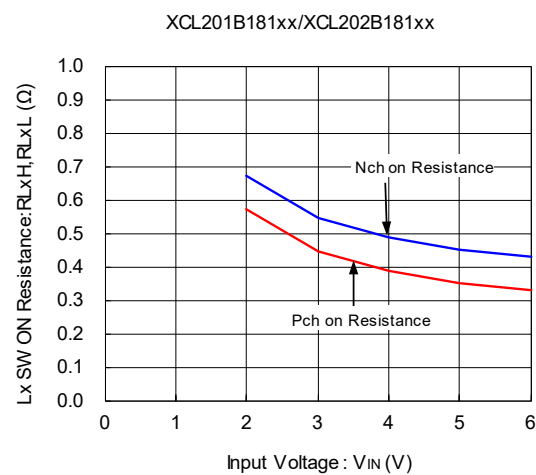
(10) "Pch / Nch" Driver on Resistance vs. Input Voltage
