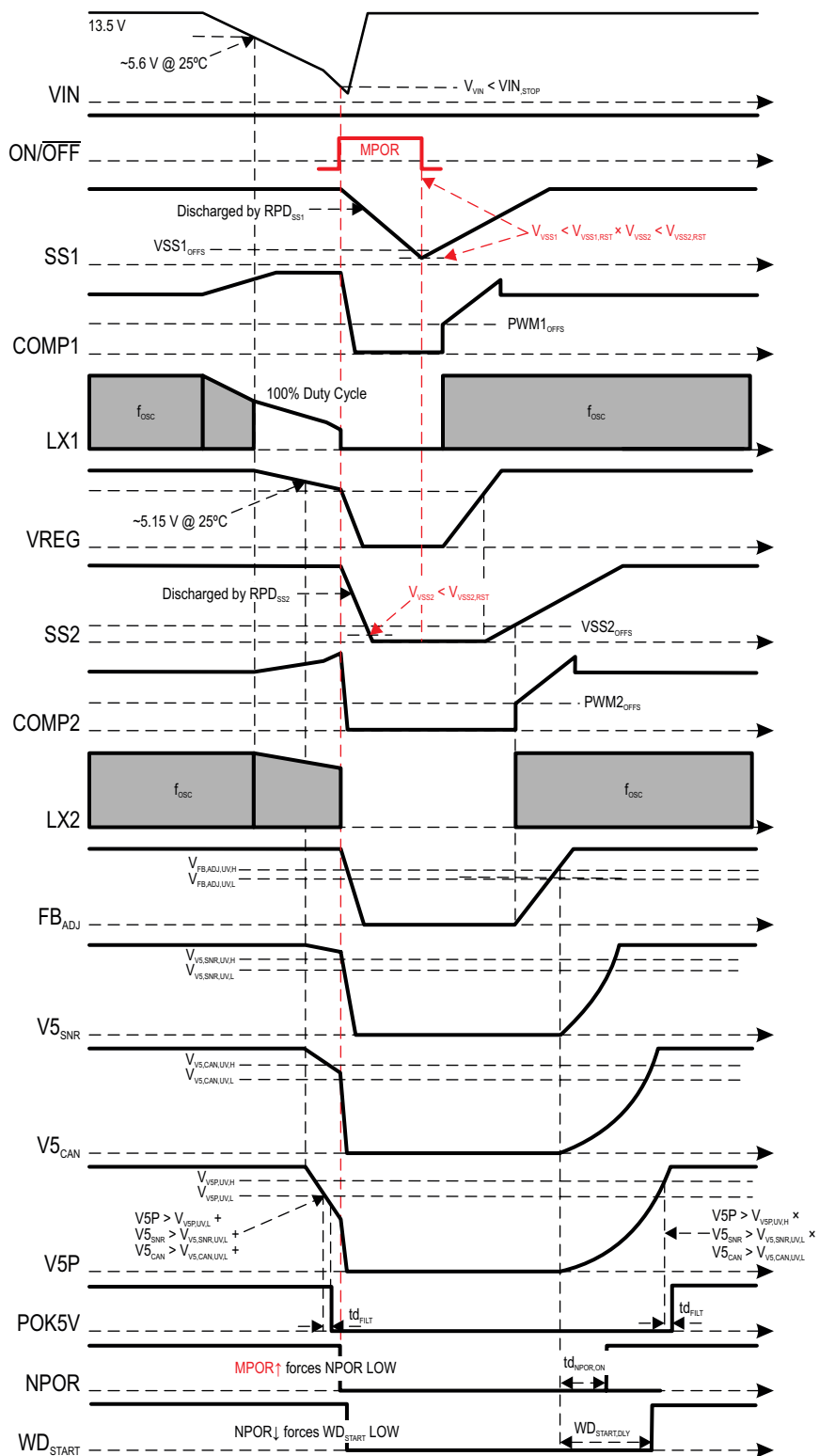
Figure 13: Input Voltage (VIN) Undervoltage, V_{VIN} < V_{VIN\_STOP}
