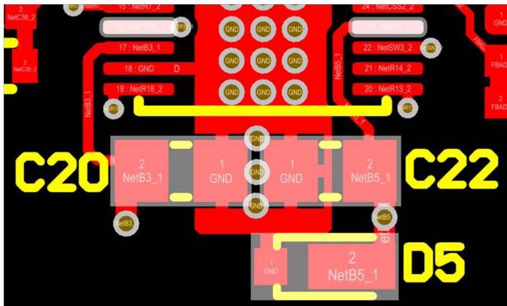
Figure 30: PCB Layout #8
