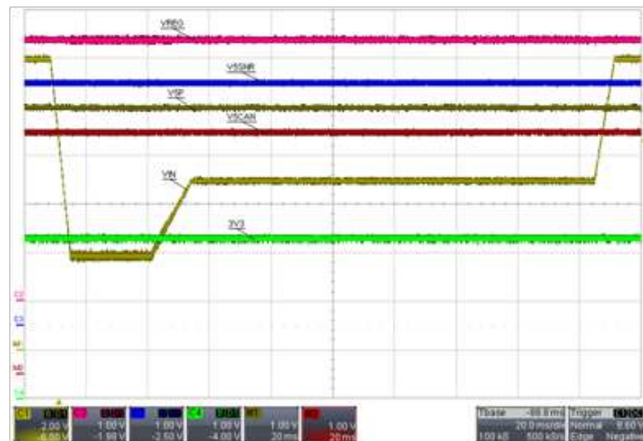
Figure 1: Buck-Boost Performance with Relatively Fast V_{IN} Transition Times for a Representative Start/Stop Waveform
