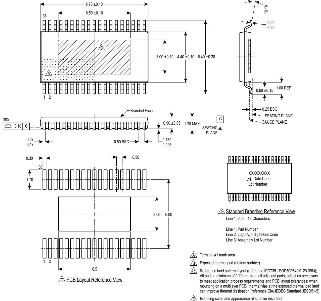
Figure 35: Package LV, 38-Pin eTSSOP
