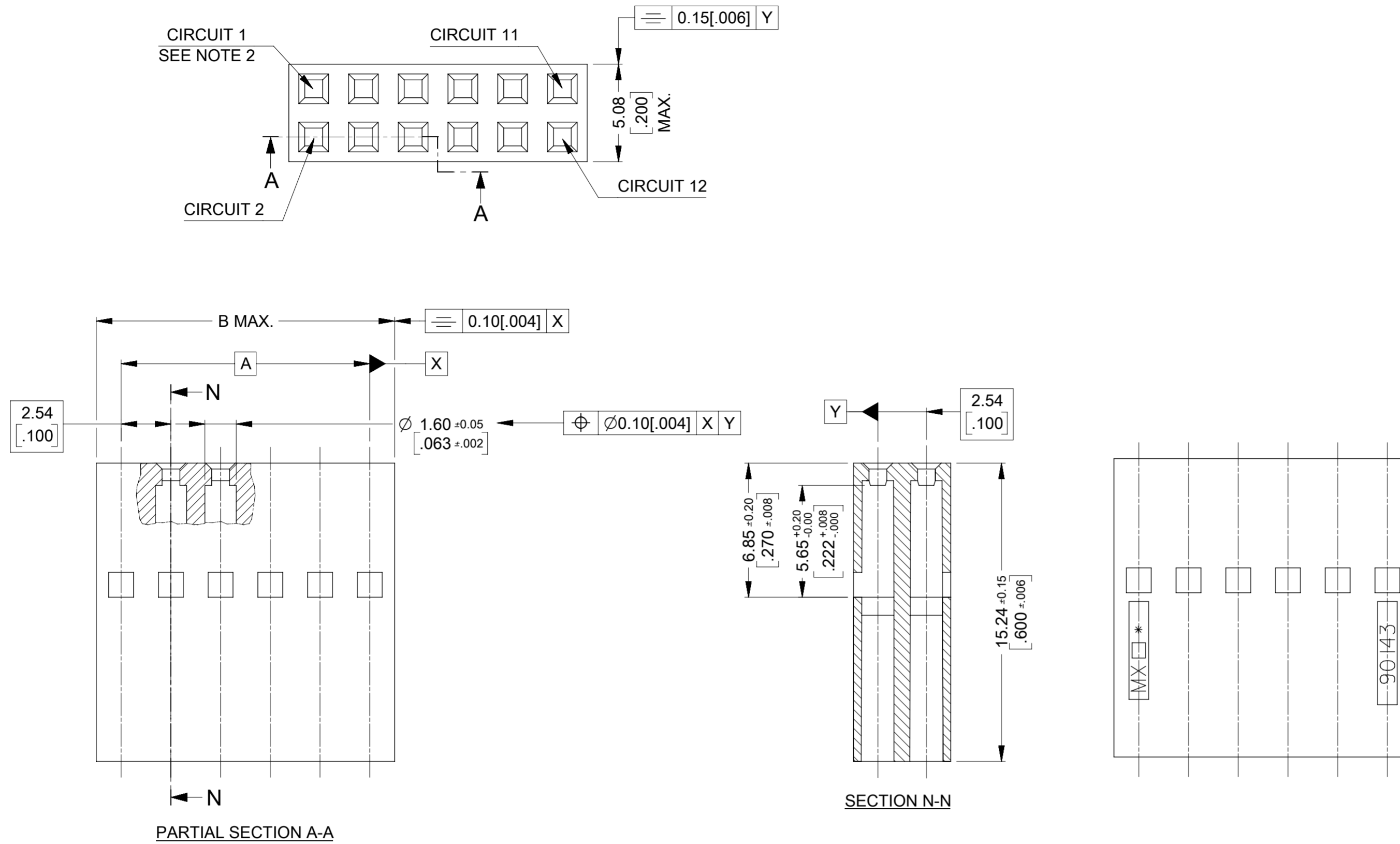
NO POLARISING BUTTON VERSION (90143-*0** VERSION)
