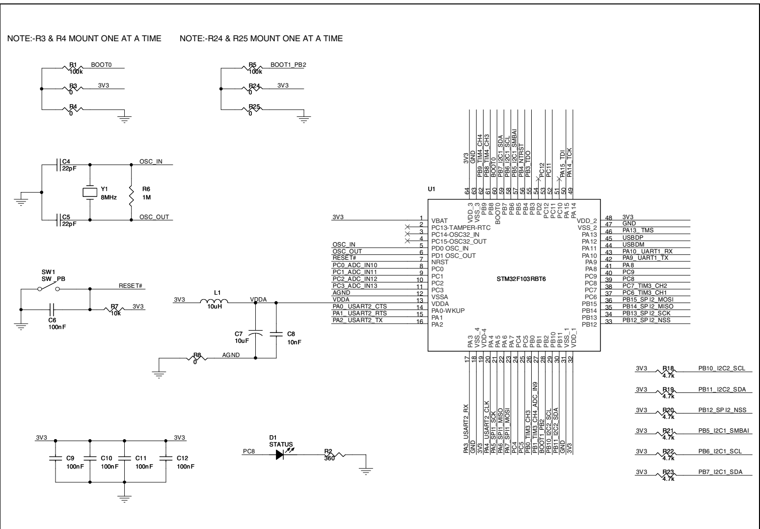
Figure 1. Microcontroller section
