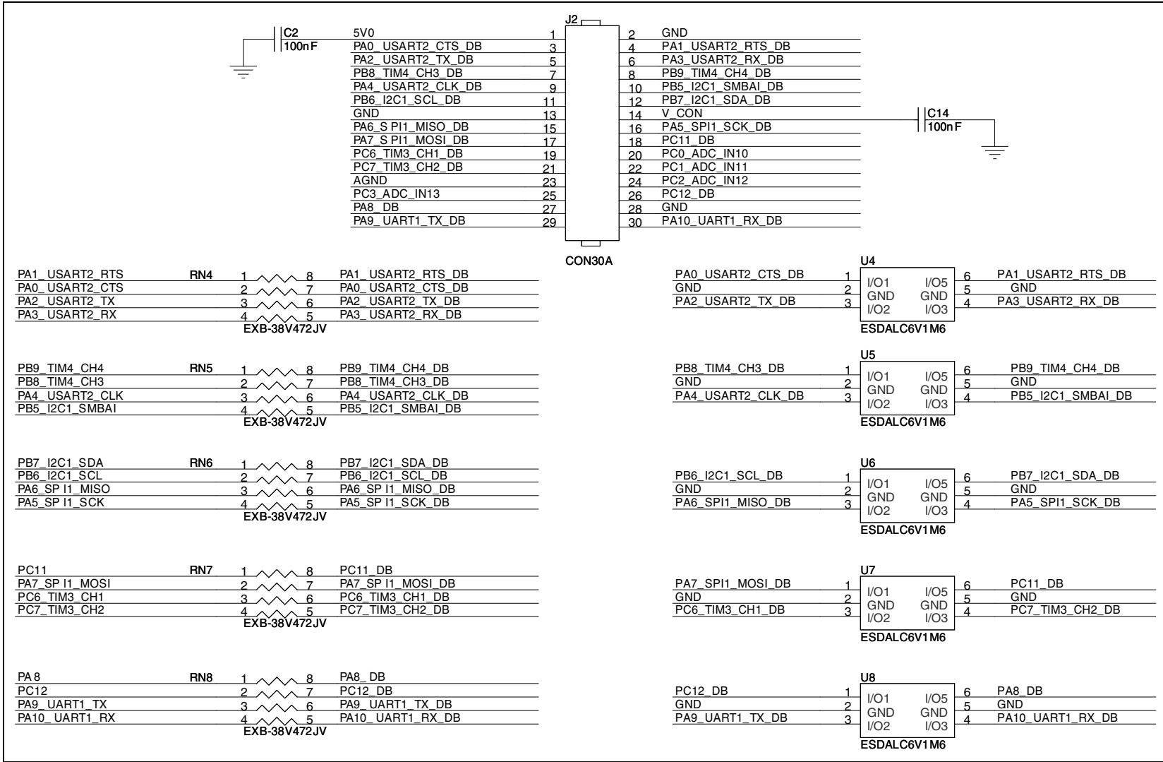
Figure 2. 30 pin COM interface
