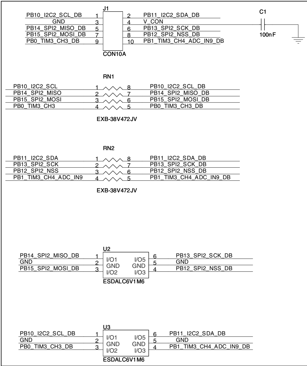
Figure 3. 10 pin COM interface
