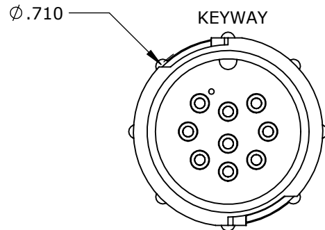
W5280-9PG-P-3XX SHOWN MATING VIEW
