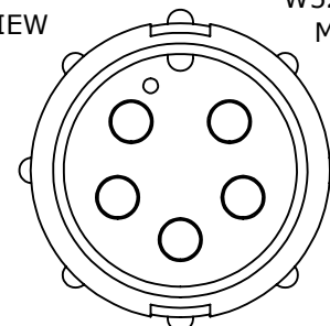
W5380-5PG-P-3XX MATING VIEW
