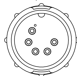
W5280-5PG-P-3XX MATING VIEW
