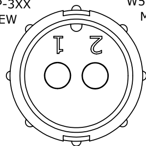
W5180-2PG-P-3XX MATING VIEW
