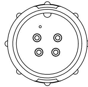
W5280-4PG-P-3XX MATING VIEW
