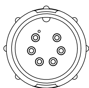
W5280-6PG-P-3XX MATING VIEW
