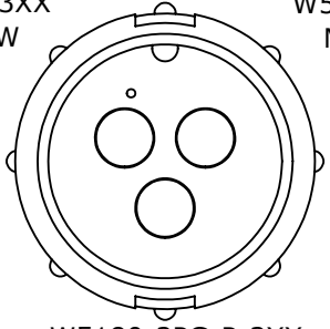
W5180-3PG-P-3XX MATING VIEW
