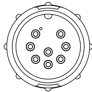
W5280-8PG-P-3XX MATING VIEW
