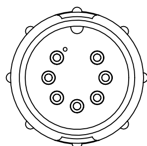
W5280-7PG-P-3XX MATING VIEW
