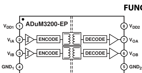
Figure 1. ADuM3200-EP Functional Block Diagram
