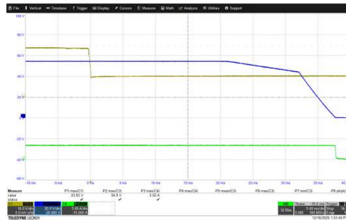
Hold Up/Interruption Time: Measured hold up time with 54Vo/180W Ch1: Vin Ch3: Vout Ch4: Iout (NOTE: for models with Hold Up option)
