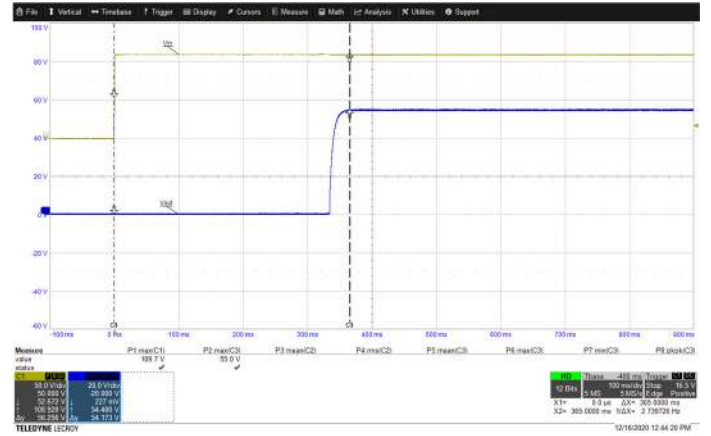
Hold Up/Interruption Time: Measured hold up time with 54Vo/300W Ch1: Vin Ch3: Vout Ch4: Iout (NOTE: for models with Hold Up option)
