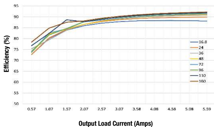
Efficiency vs Line and Load
