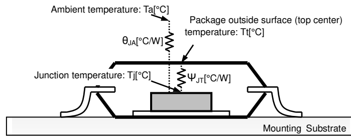
Figure 48. Thermal Resistance Model of Surface Mount
