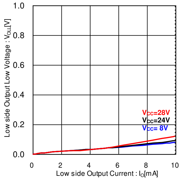
Figure 17. Low side Output Low Voltage vs Low side Output Current ( T_a=25^{\circ}C )
