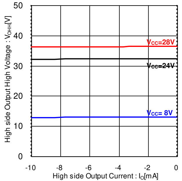
Figure 11. High side Output High Voltage vs High side Output Current ( T_a=25^{\circ}C )
