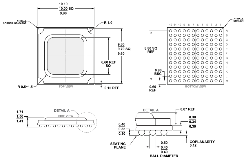
COMPLIANT TO JEDEC STANDARDS MO-275-EEAB-1. Figure 86. 144-Ball Ball Grid Array, Thermally Enhanced [BGA_ED] (BP-144-1) Dimensions shown in millimeters
