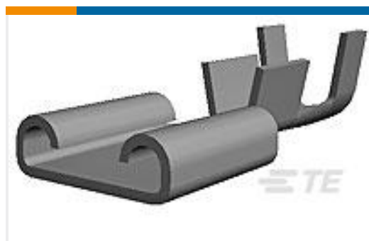
TE Part #1-160301-9 250 FASTON,REC.,10-12 AWG,PHBZ
