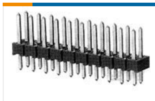
TE Part #9-146250-0 80 MODII HDR DRST B/A .100CL
