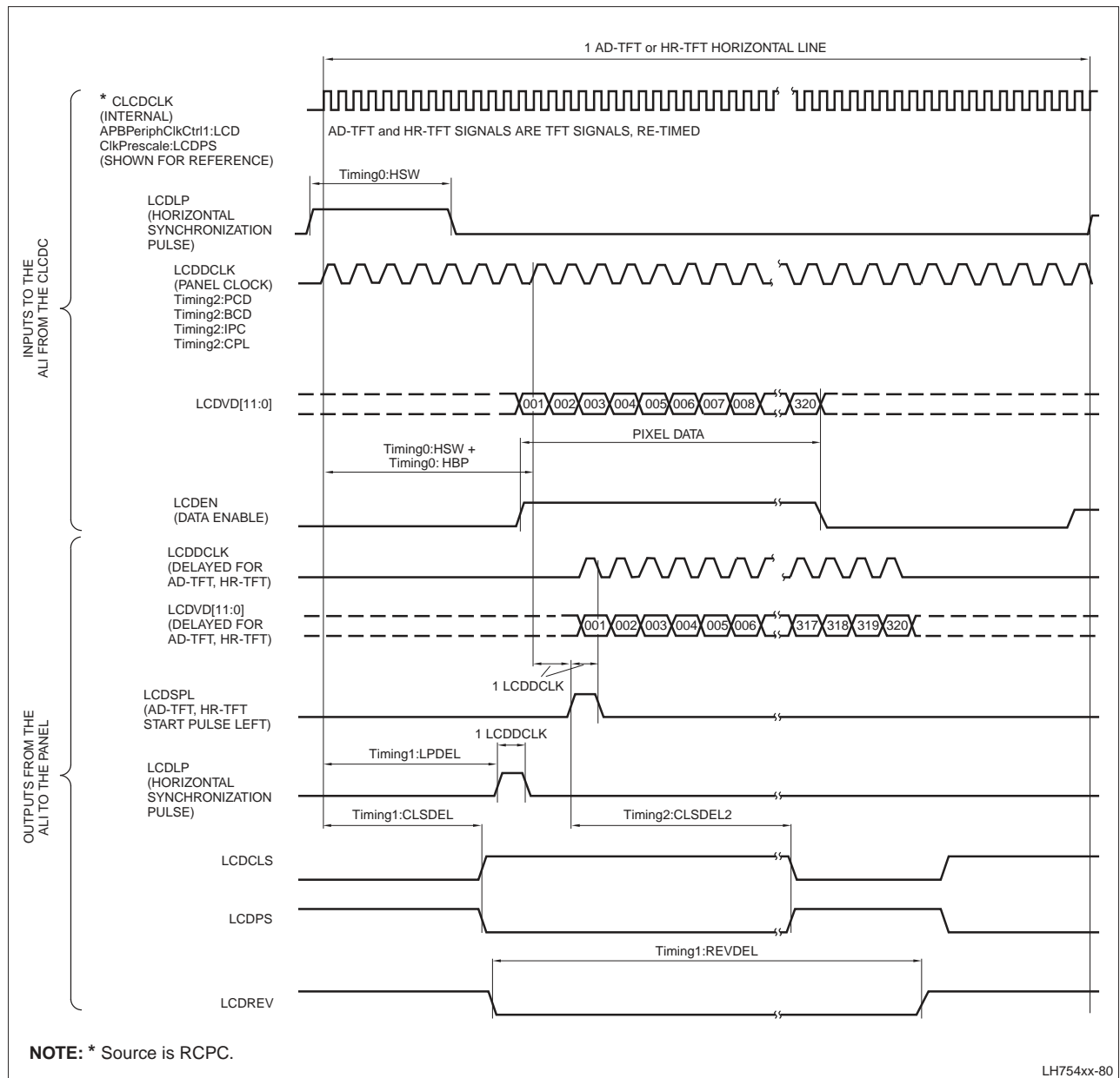
Figure 19. AD-TFT, HR-TFT Horizontal Timing Diagram
