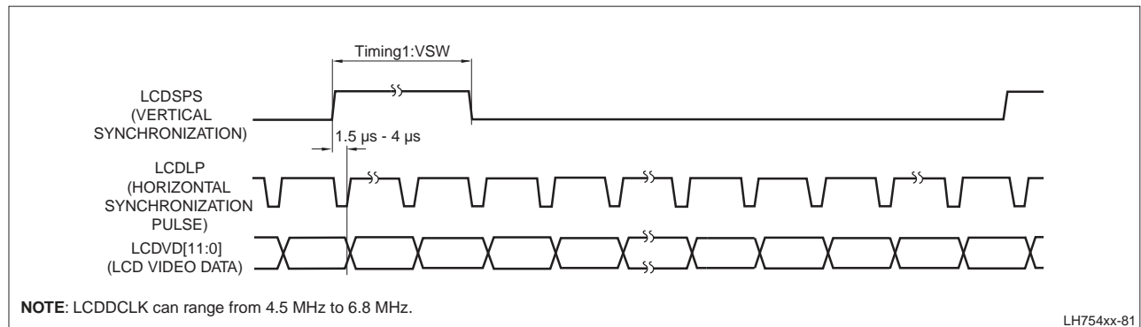
Figure 20. AD-TFT, HR-TFT Vertical Timing Diagram
