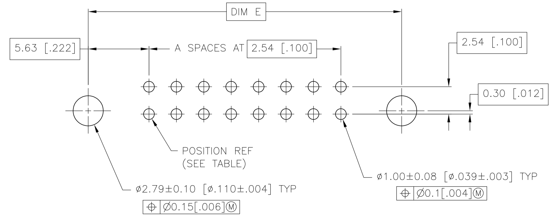
RECOMMENDED PC BOARD LAYOUT
