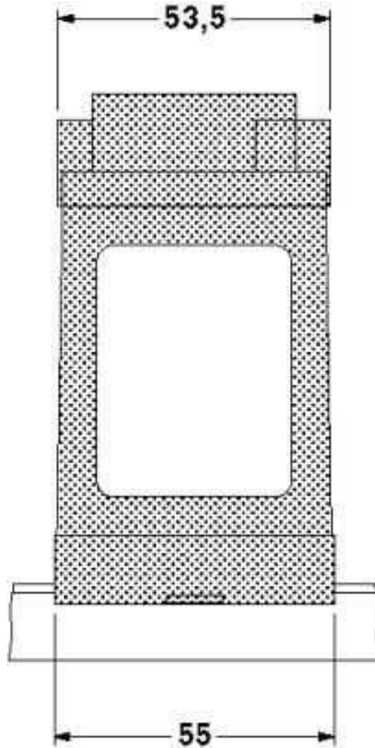
Dimensioned drawing
