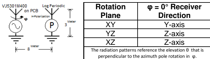
Figure 3 VJ5301M400 PCB mounting and coordinate directions
