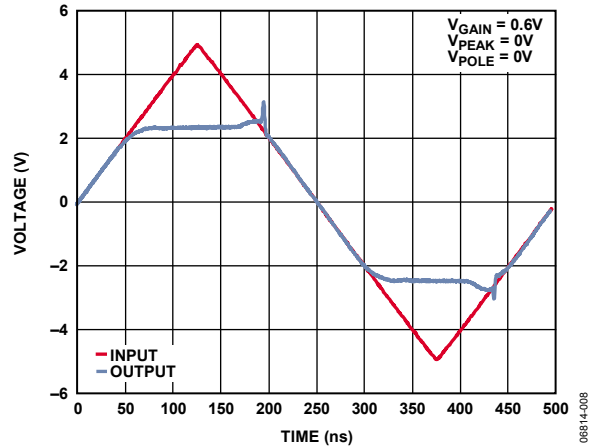
Figure 10. Overdrive Recovery
