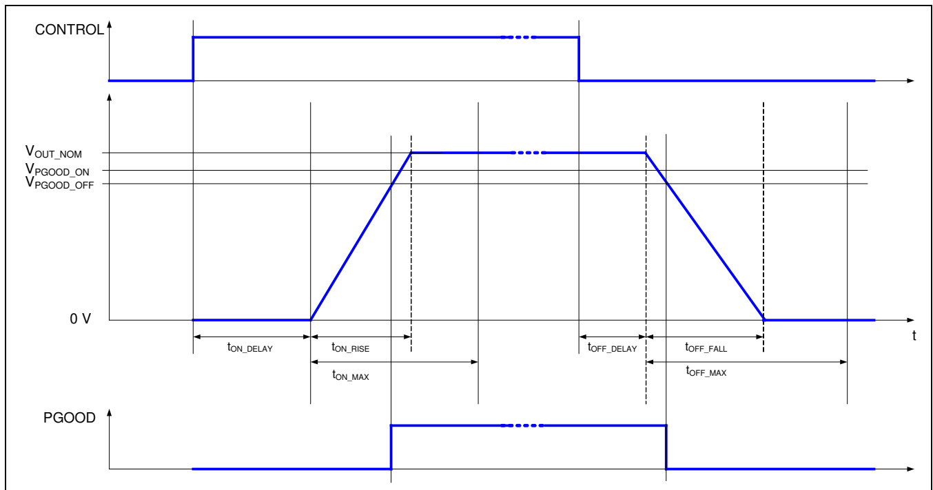
Figure 3.2 Power Sequencing
