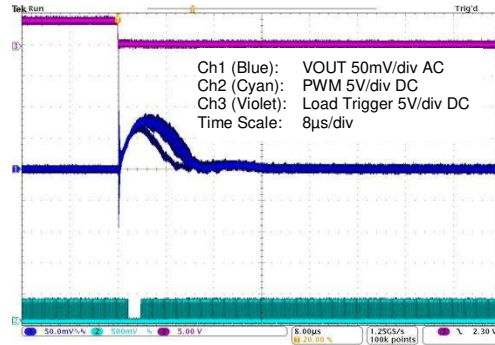
Figure 5.29 ZSPM1502 with Comp1; 15A to 5A Load Step; and Max. Capacitance
