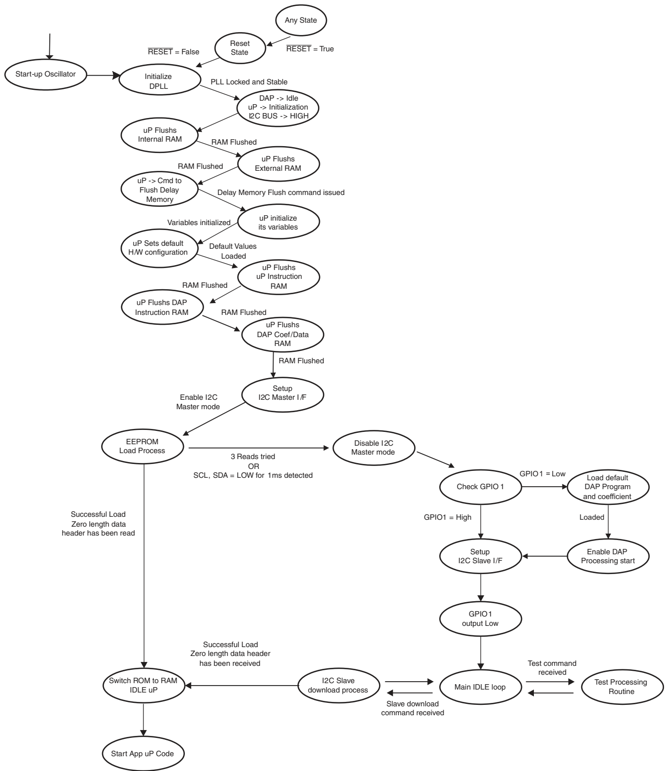
Figure 17. Boot-Up Sequence
