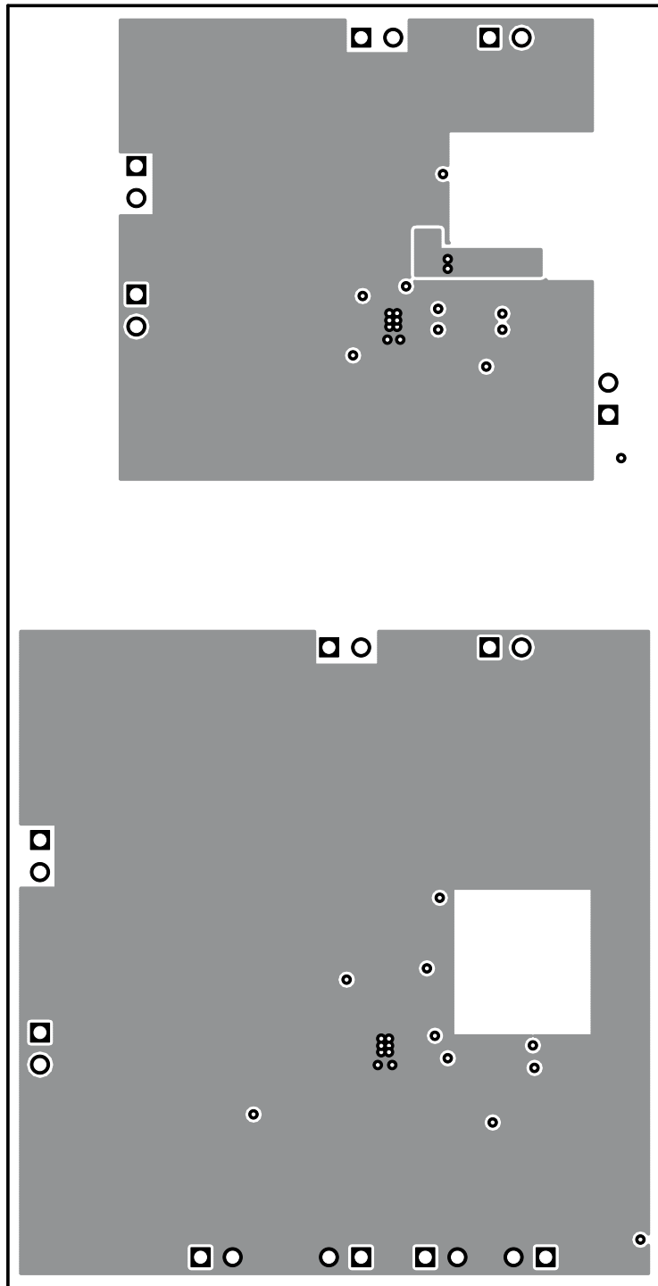
Figure 18. Layer 2 Routing
