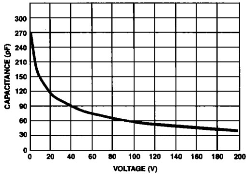
FIGURE 3. TYPICAL CAPACITANCE vs VOLTAGE FOR SGT27B27
