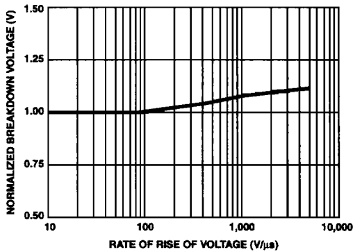
FIGURE 5. NORMALIZED V_{BO} vs dv/dt FOR ALL TYPES
