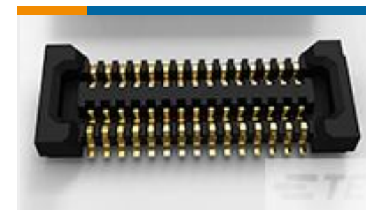
TE Part #1-2201197-0 0.4 STACKING CONN H0.98 REC ASSEMBLY
