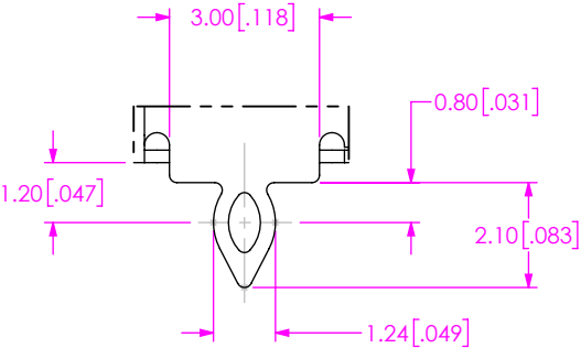
DETAIL 'H' SCALE 6 : 1
