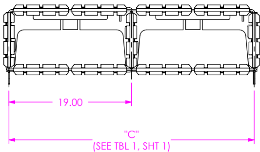
FIG 8 QSFP-1-2-S-N-F SHOWN (DIFFERENT AS SHOWN, OTHERWISE SAME AS FIGS 1 & 4)
