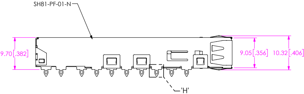
FIG 7 QSFP-1-1-S-N-F SHOWN (SAME AS FIG 1, EXCEPT AS SHOWN)
