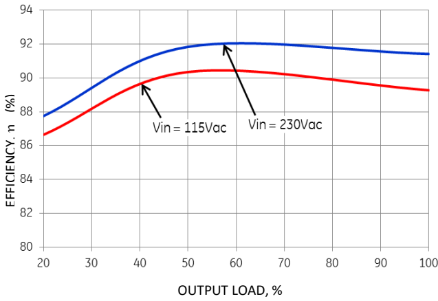
Figure 1. Converter Efficiency versus % Load.
