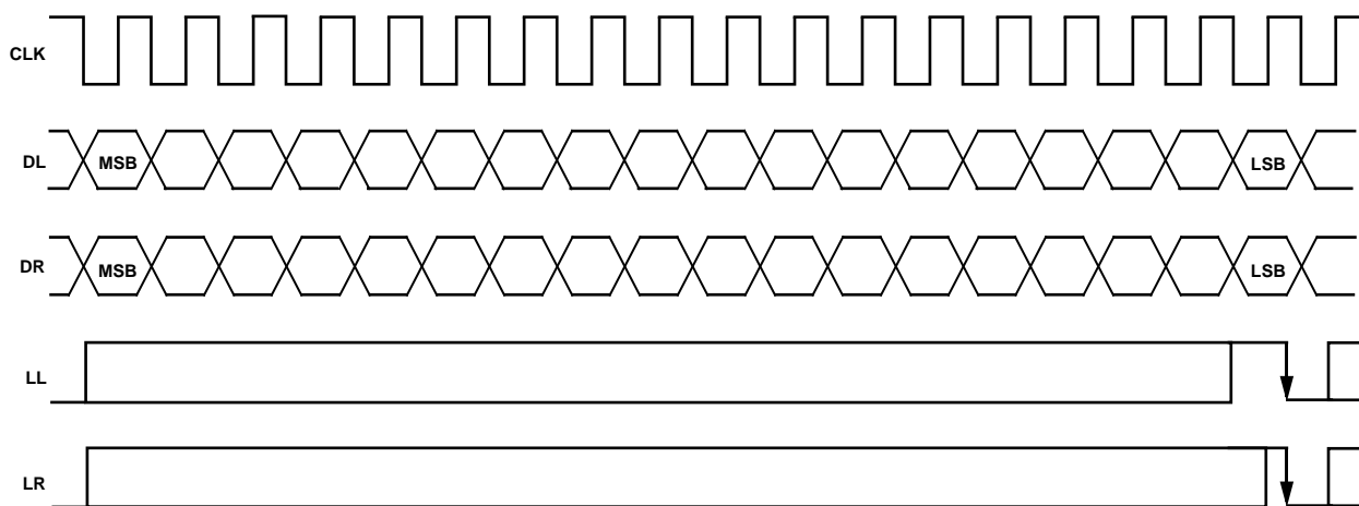
Figure 9. Control Signals
