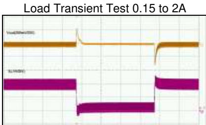
Time-500μs/div
