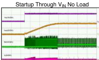
Time-5ms/div
