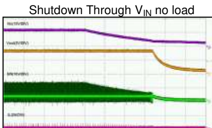
Time-20ms/div
