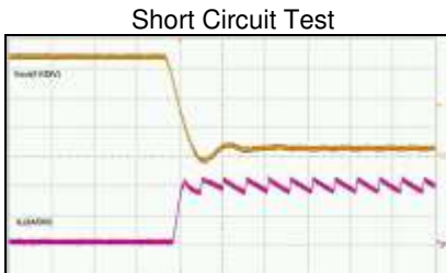
Time-20μs/div
