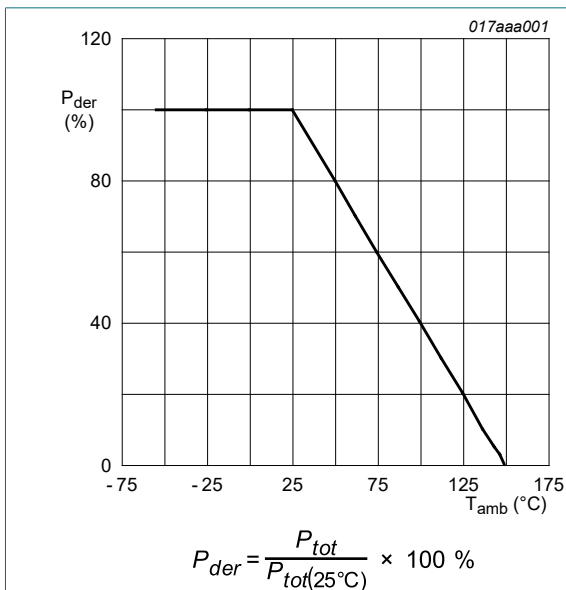
Fig. 1. Normalized total power dissipation as a function of ambient temperature
