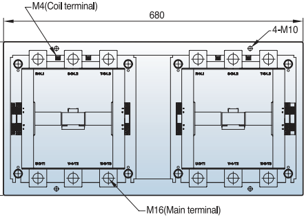
CC500 ~ CC800 reversing combination shown with aux contacts
