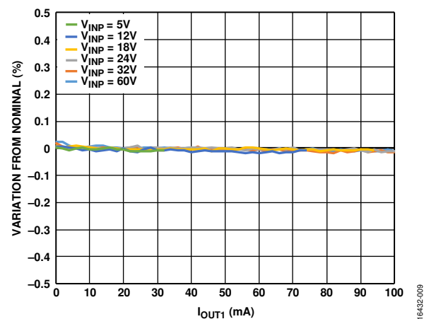
Figure 9. Flyback Regulator Output Load Regulation, V_{OUT1} = 24\text{ V} , T_A = 25^\circ\text{C} , Nominal = V_{OUT1} at 20 mA Load
