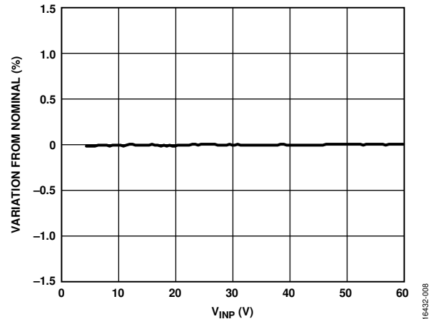
Figure 8. Flyback Regulator Output Line Regulation, Flyback Regulator Output Voltage ( V_{OUT1} ) = 24 V, Flyback Regulator Output Current ( I_{OUT1} ) = 20 mA, T_A = 25^\circ\text{C} , Load Regulation, Nominal = V_{OUT1} at 24 V Input Supply
