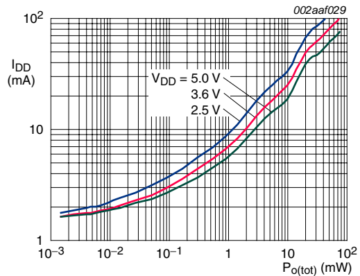
Fig 14. Supply current versus total output power
