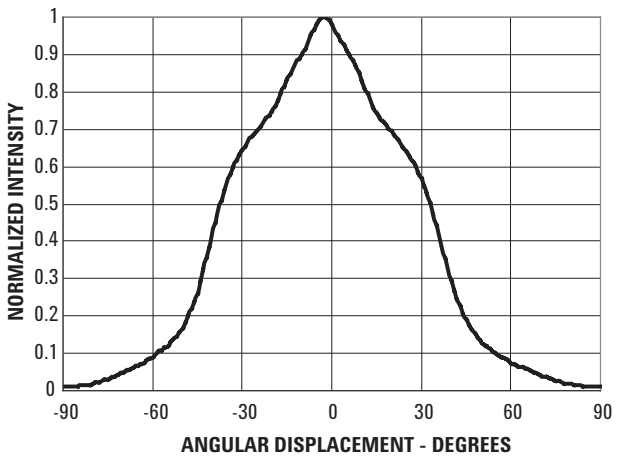
Figure 6. Representative Spatial Radiation Pattern for the — major axis
