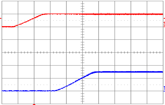
Fig. 1.5V.5: Turn-on transient for V_{out} = 1.5\text{ V} with application of V_{in} at full rated load current (resistive) and 47 \mu\text{F} external capacitance at V_{in} = 5\text{ V} . Top trace: V_{in} (5 V/div.); Bottom trace: output voltage (1 V/div.); Time scale: 2 ms/div.
