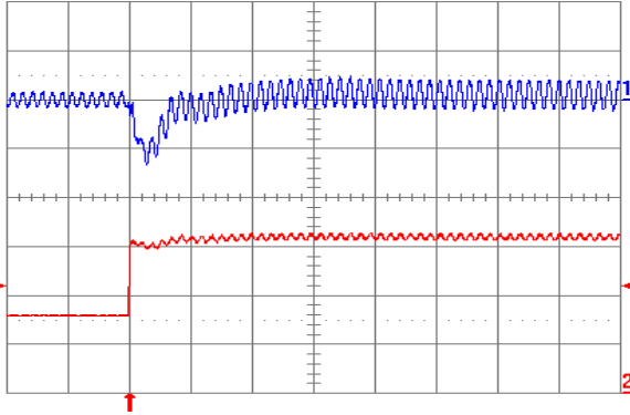
Fig. 2.0V.7: Output voltage response for V_{out} = 2.0\text{ V} to positive load current step change from 3 A to 6 A with slew rate of 5\text{ A}/\mu\text{s} at V_{in} = 5\text{ V} . Top trace: output voltage (100 mV/div.); Bottom trace: load current (2 A/div.). C_o = 47\text{ }\mu\text{F} ceramic + 1\text{ }\mu\text{F} ceramic. Time scale: 20\text{ }\mu\text{s}/\text{div} .
