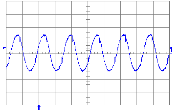
Fig. 1.8V.6: Output voltage ripple (20 mV/div.) at full rated load current into a resistive load with external capacitance 10\ \mu\text{F} ceramic + 1\ \mu\text{F} ceramic and V_{in} = 5\text{ V} for V_{out} = 1.8\text{ V} . Time scale: 2 \mu\text{s} /div.
