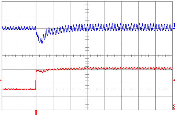
Fig. 1.2V.6: Output voltage response for V_{out} = 1.2\text{ V} to positive load current step change from 3 A to 6 A with slew rate of 5\text{ A}/\mu\text{s} at V_{in} = 5\text{ V} . Top trace: output voltage (100 mV/div.); Bottom trace: load current (2 A/div.). C_o = 47\text{ }\mu\text{F} ceramic + 1\text{ }\mu\text{F} ceramic. Time scale: 20\text{ }\mu\text{s}/\text{div} .
