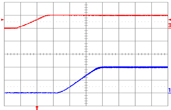
Fig. 2.0V.5: Turn-on transient for V_{out} = 2.0\text{ V} with application of V_{in} at full rated load current (resistive) and 47\text{ }\mu\text{F} external capacitance at V_{in} = 5\text{ V} . Top trace: V_{in} (5 V/div.); Bottom trace: output voltage (1 V/div.); Time scale: 2 ms/div.
