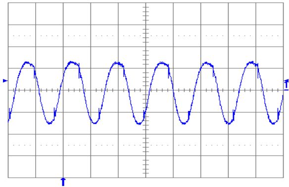
Fig. 2.5V.6: Output voltage ripple (20 mV/div.) at full rated load current into a resistive load with external capacitance 10\text{ }\mu\text{F} ceramic + 1\text{ }\mu\text{F} ceramic and V_{in} = 5\text{ V} for V_{out} = 2.5\text{ V} . Time scale: 2 \mu\text{s} /div.
