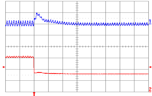
Fig. 1.0V.8: Output voltage response for V_{out} = 1.0\text{ V} to negative load current step change from 6 A to 3 A with slew rate of -5\text{ A}/\mu\text{s} at V_{in} = 5\text{ V} . Top trace: output voltage (100 mV/div.); Bottom trace: load current (2 A/div.). C_o = 47\ \mu\text{F} ceramic + 1\ \mu\text{F} ceramic. Time scale: 20 \mu\text{s} /div.
