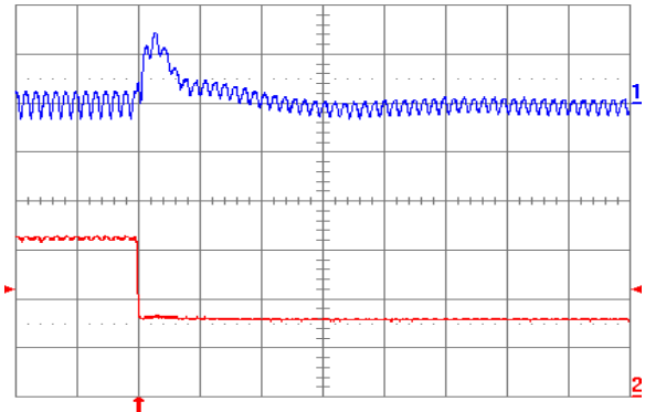
Fig. 3.3V.8: Output voltage response for V_{out} = 3.3\text{ V} to negative load current step change from 6 A to 3 A with slew rate of -5\text{ A}/\mu\text{s} at V_{in} = 5\text{ V} . Top trace: output voltage (100 mV/div.); Bottom trace: load current (2 A/div.). C_o = 47\ \mu\text{F} ceramic + 1\ \mu\text{F} ceramic. Time scale: 20 \mu\text{s} /div.
