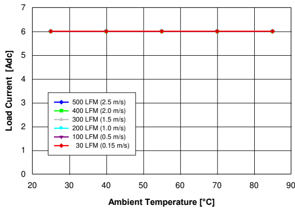
Fig. 3.3V.1: Available load current vs. ambient temperature and airflow rates for V_{out} = 3.3\ \text{V} converter mounted vertically with V_{in} = 5\ \text{V} , air flowing from pin 5 to pin 1, and maximum MOSFET temperature \leq 120^\circ\text{C} .
