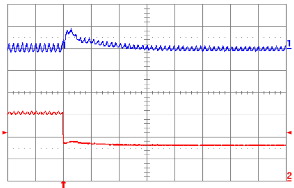
Fig. 0.7525V.8: Output voltage response for V_{out} = 0.7525\text{ V} to negative load current step change from 6 A to 3 A with slew rate of -5 A/ \mu\text{s} at V_{in} = 5\text{ V} . Top trace: output voltage (100 mV/div.); Bottom trace: load current (2 A/div.). C_o = 47\text{ }\mu\text{F} ceramic + 1 \mu\text{F} ceramic. Time scale: 20 \mu\text{s} /div.
