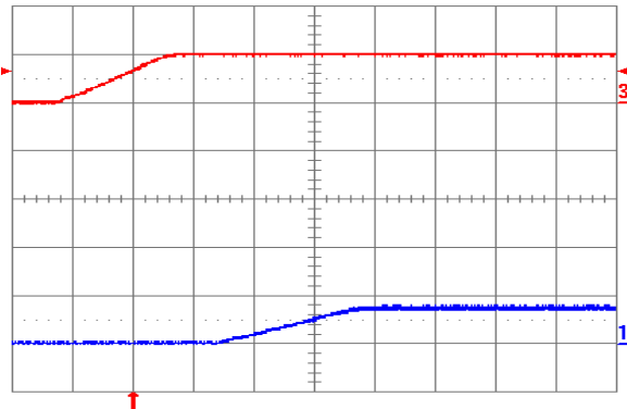
Fig. 0.7525V.4: Turn-on transient for V_{out} = 0.7525\text{ V} with application of V_{in} at full rated load current (resistive) and 47 \mu\text{F} external capacitance at V_{in} = 5\text{ V} . Top trace: V_{in} (5 V/div.); Bottom trace: output voltage (1 V/div.); Time scale: 2 ms/div.
