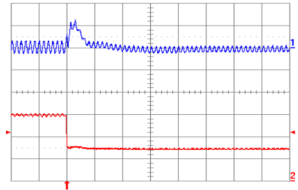
Fig. 1.8V.8: Output voltage response for V_{out} = 1.8\text{ V} to negative load current step change from 6 A to 3 A with slew rate of -5\text{ A}/\mu\text{s} at V_{in} = 5\text{ V} . Top trace: output voltage (100 mV/div.); Bottom trace: load current (2 A/div.). C_o = 47\ \mu\text{F} ceramic + 1\ \mu\text{F} ceramic. Time scale: 20 \mu\text{s} /div.
