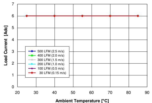
Fig. 2.5V.2: Available load current vs. ambient temperature and airflow rates for V_{out} = 2.5\text{ V} converter mounted horizontally with V_{in} = 5\text{ V} , air flowing from pin 5 to pin 1, and maximum MOSFET temperature \leq 120\text{ }^\circ\text{C} .
