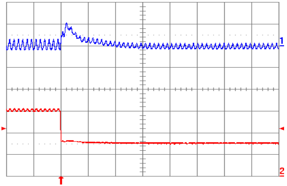
Fig. 1.2V.8: Output voltage response for V_{out} = 1.2\text{ V} to negative load current step change from 6 A to 3 A with slew rate of -5\text{ A}/\mu\text{s} at V_{in} = 5\text{ V} . Top trace: output voltage (100 mV/div.); Bottom trace: load current (2 A/div.). C_o = 47\text{ }\mu\text{F} ceramic + 1\text{ }\mu\text{F} ceramic. Time scale: 20\text{ }\mu\text{s}/\text{div} .
