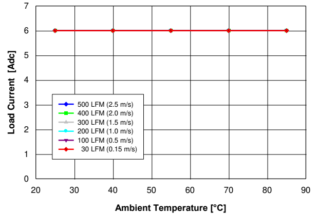
Fig. 2.0V.2: Available load current vs. ambient temperature and airflow rates for V_{out} = 2.0\text{ V} converter mounted horizontally with V_{in} = 5\text{ V} , air flowing from pin 5 to pin 1, and maximum MOSFET temperature \leq 120\text{ }^{\circ}\text{C} .
