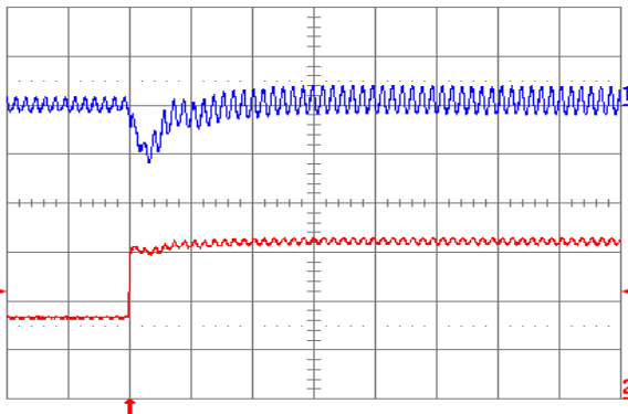
Fig. 1.5V.7: Output voltage response for V_{out} = 1.5\text{ V} to positive load current step change from 3 A to 6 A with slew rate of 5 A/ \mu\text{s} at V_{in} = 5\text{ V} . Top trace: output voltage (100 mV/div.); Bottom trace: load current (2 A/div.). C_o = 47\text{ }\mu\text{F} ceramic + 1 \mu\text{F} ceramic. Time scale: 20 \mu\text{s} /div.
