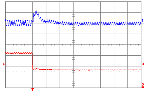
Fig. 1.5V.8: Output voltage response for V_{out} = 1.5\text{ V} to negative load current step change from 6 A to 3 A with slew rate of -5 A/ \mu\text{s} at V_{in} = 5\text{ V} . Top trace: output voltage (100 mV/div.); Bottom trace: load current (2 A/div.). C_o = 47\text{ }\mu\text{F} ceramic + 1 \mu\text{F} ceramic. Time scale: 20 \mu\text{s} /div.
