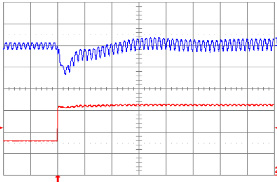
Fig. 3.3V.7: Output voltage response for V_{out} = 3.3\text{ V} to positive load current step change from 3 A to 6 A with slew rate of 5\text{ A}/\mu\text{s} at V_{in} = 5\text{ V} . Top trace: output voltage (100 mV/div.); Bottom trace: load current (2 A/div.). C_o = 47\ \mu\text{F} ceramic + 1\ \mu\text{F} ceramic. Time scale: 20 \mu\text{s} /div.
