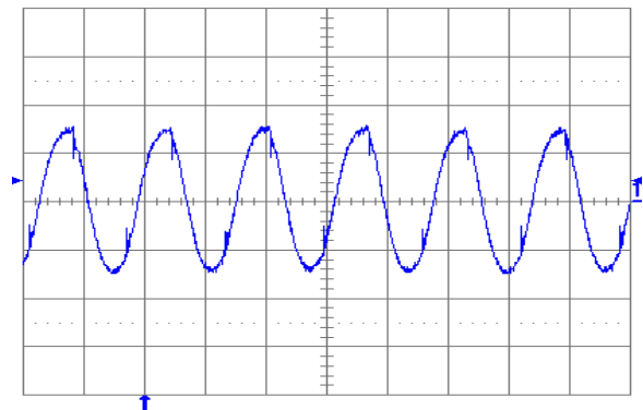
Fig. 2.0V.6: Output voltage ripple (20 mV/div.) at full rated load current into a resistive load with external capacitance 10\text{ }\mu\text{F} ceramic + 1\text{ }\mu\text{F} ceramic and V_{in} = 5\text{ V} for V_{out} = 2.0\text{ V} . Time scale: 2 μs/div.
