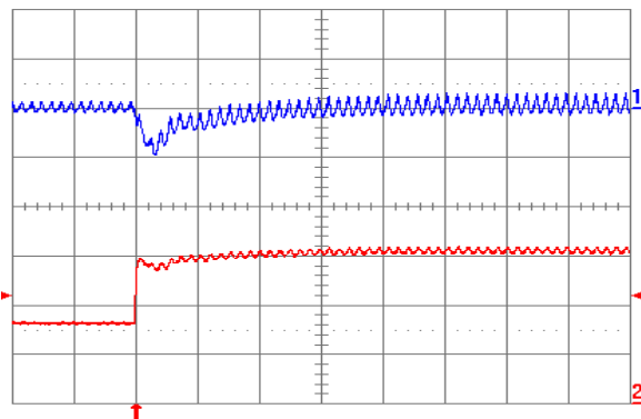
Fig. 0.7525V.7: Output voltage response for V_{out} = 0.7525\text{ V} to positive load current step change from 3 A to 6 A with slew rate of 5 A/ \mu\text{s} at V_{in} = 5\text{ V} . Top trace: output voltage (100 mV/div.); Bottom trace: load current (2 A/div.). C_o = 47\text{ }\mu\text{F} ceramic + 1 \mu\text{F} ceramic. Time scale: 20 \mu\text{s} /div.
