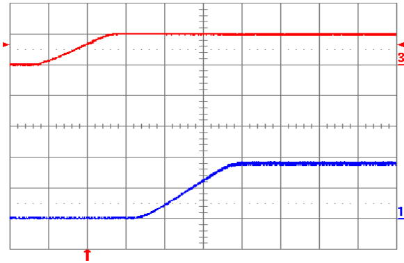
Fig. 1.8V.5: Turn-on transient for V_{out} = 1.8\text{ V} with application of V_{in} at full rated load current (resistive) and 47\ \mu\text{F} external capacitance at V_{in} = 5\text{ V} . Top trace: V_{in} (5 V/div.); Bottom trace: output voltage (1 V/div.); Time scale: 2 ms/div.
