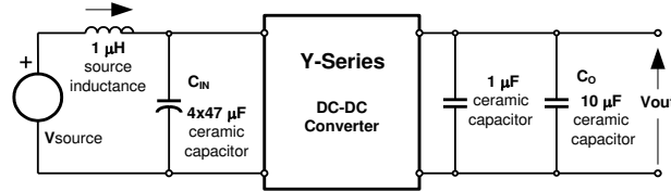
Fig. F: Test setup for measuring input reflected-ripple currents, i_s and output voltage ripple.
