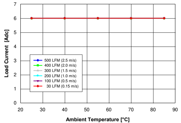
Fig. 1.0V.2: Available load current vs. ambient temperature and airflow rates for V_{out} = 1.0\text{ V} converter mounted horizontally with V_{in} = 5\text{ V} , air flowing from pin 5 to pin 1, and maximum MOSFET temperature \leq 120\text{ }^\circ\text{C} .
