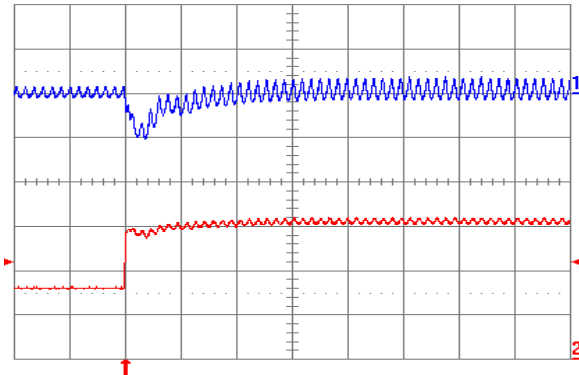
Fig. 1.0V.7: Output voltage response for V_{out} = 1.0\text{ V} to positive load current step change from 3 A to 6 A with slew rate of 5\text{ A}/\mu\text{s} at V_{in} = 5\text{ V} . Top trace: output voltage (100 mV/div.); Bottom trace: load current (2 A/div.). C_o = 47\ \mu\text{F} ceramic + 1\ \mu\text{F} ceramic. Time scale: 20 \mu\text{s} /div.
