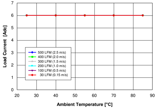
Fig. 2.0V.1: Available load current vs. ambient temperature and airflow rates for V_{out} = 2.0\text{ V} converter mounted vertically with V_{in} = 5\text{ V} , air flowing from pin 5 to pin 1, and maximum MOSFET temperature \leq 120\text{ }^{\circ}\text{C} .
