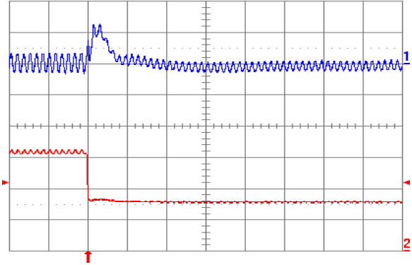
Fig. 2.0V.8: Output voltage response for V_{out} = 2.0\text{ V} to negative load current step change from 6 A to 3 A with slew rate of -5\text{ A}/\mu\text{s} at V_{in} = 5\text{ V} . Top trace: output voltage (100 mV/div.); Bottom trace: load current (2 A/div.). C_o = 47\text{ }\mu\text{F} ceramic + 1\text{ }\mu\text{F} ceramic. Time scale: 20\text{ }\mu\text{s}/\text{div} .
