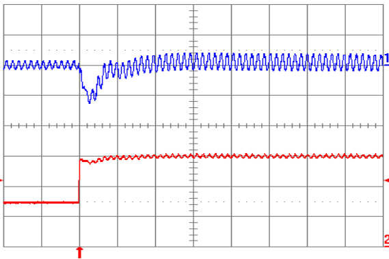
Fig. 1.8V.7: Output voltage response for V_{out} = 1.8\text{ V} to positive load current step change from 3 A to 6 A with slew rate of 5\text{ A}/\mu\text{s} at V_{in} = 5\text{ V} . Top trace: output voltage (100 mV/div.); Bottom trace: load current (2 A/div.). C_o = 47\ \mu\text{F} ceramic + 1\ \mu\text{F} ceramic. Time scale: 20 \mu\text{s} /div.
