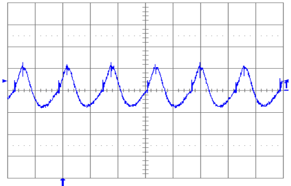
Fig. 0.7525V.5: Output voltage ripple (20 mV/div.) at full rated load current into a resistive load with external capacitance 10 \mu\text{F} ceramic + 1 \mu\text{F} ceramic and V_{in} = 5\text{ V} for V_{out} = 0.7525\text{ V} . Time scale: 2 \mu\text{s} /div.
