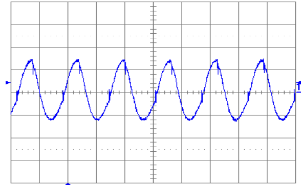
Fig. 1.5V.6: Output voltage ripple (20 mV/div.) at full rated load current into a resistive load with external capacitance 10 \mu\text{F} ceramic + 1 \mu\text{F} ceramic and V_{in} = 5\text{ V} for V_{out} = 1.5\text{ V} . Time scale: 2 \mu\text{s} /div.
