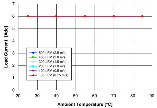
Fig. 3.3V.2: Available load current vs. ambient temperature and airflow rates for V_{out} = 3.3\ \text{V} converter mounted horizontally with V_{in} = 5\ \text{V} , air flowing from pin 5 to pin 1, and maximum MOSFET temperature \leq 120^\circ\text{C} .
