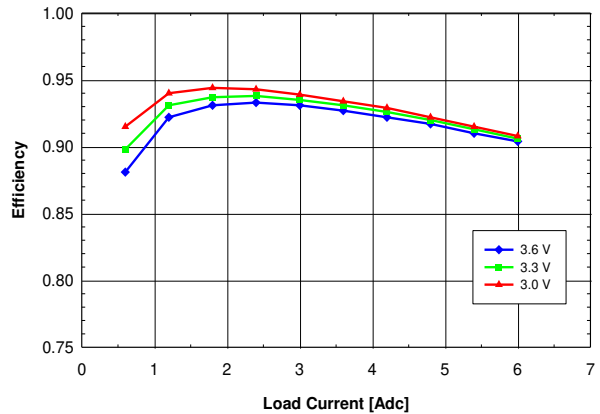
Fig. 2.0V.4: Efficiency vs. load current and input voltage for V_{out} = 2.0\text{ V} converter mounted vertically with air flowing from pin 5 to pin 1 at a rate of 200 LFM (1 m/s) and T_a = 25\text{ }^{\circ}\text{C} .
