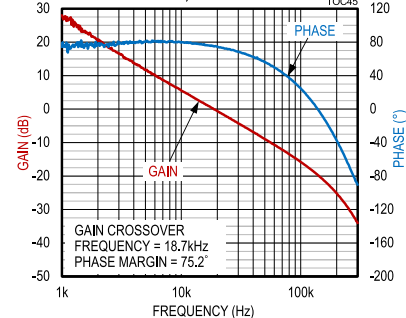
MAX17579, -15V OUTPUT, BODE PLOT, FIGURE 8 CIRCUIT TOC45
