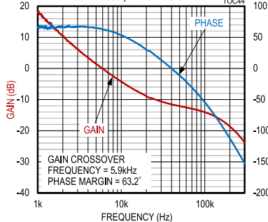
MAX17579, -15V OUTPUT, BODE PLOT, FIGURE 8 CIRCUIT TOC44
