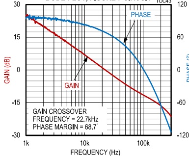
MAX17579/MAX17580, -15V OUTPUT, BODE PLOT, FIGURE 7 CIRCUIT TOC43
