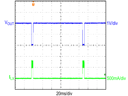
MAX17579/MAX17580, -5V OUTPUT, OVERLOAD PROTECTION FIGURE 5 CIRCUIT TOC39
