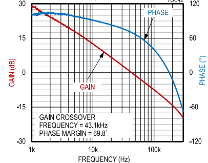
MAX17579, -5V OUTPUT, BODE PLOT, FIGURE 6 CIRCUIT TOC42
