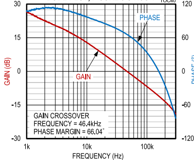
MAX17579/MAX17580, -5V OUTPUT, BODE PLOT, FIGURE 5 CIRCUIT TOC40
