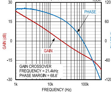
MAX17579, -5V OUTPUT, BODE PLOT, FIGURE 6 CIRCUIT TOC41
