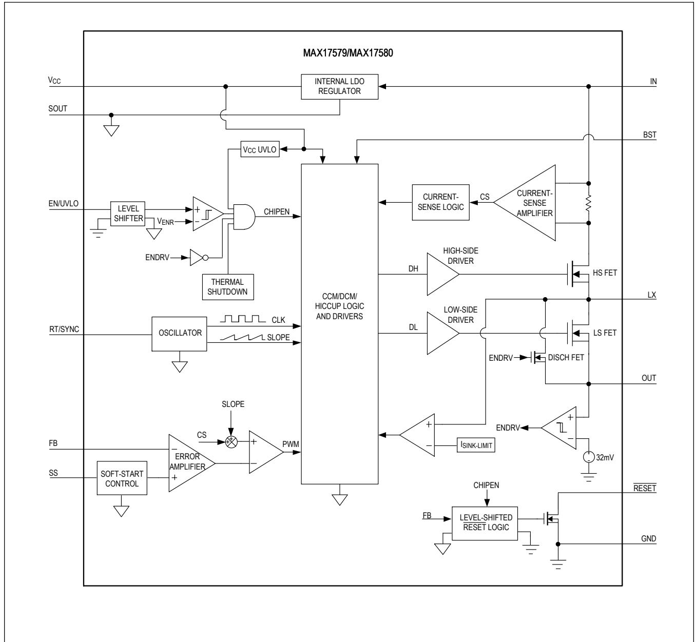
MAX17579/MAX17580 Block Diagram
