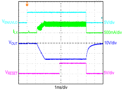
MAX17579/MAX17580, -15V OUTPUT, SOFT-START AND SHUTDOWN THROUGH EN/UVLO, FIGURE 7 CIRCUIT TOC37
