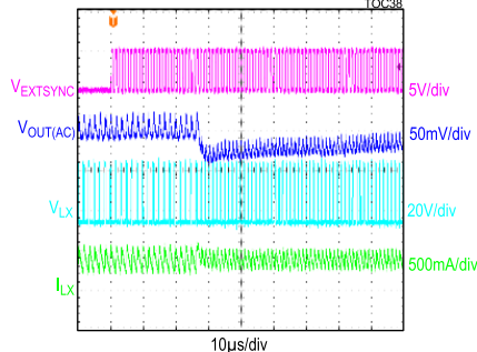
MAX17579/MAX17580, -5V OUTPUT, EXTERNAL CLOCK SYNCHRONIZATION WITH 840kHz, FIGURE 5 CIRCUIT TOC38
