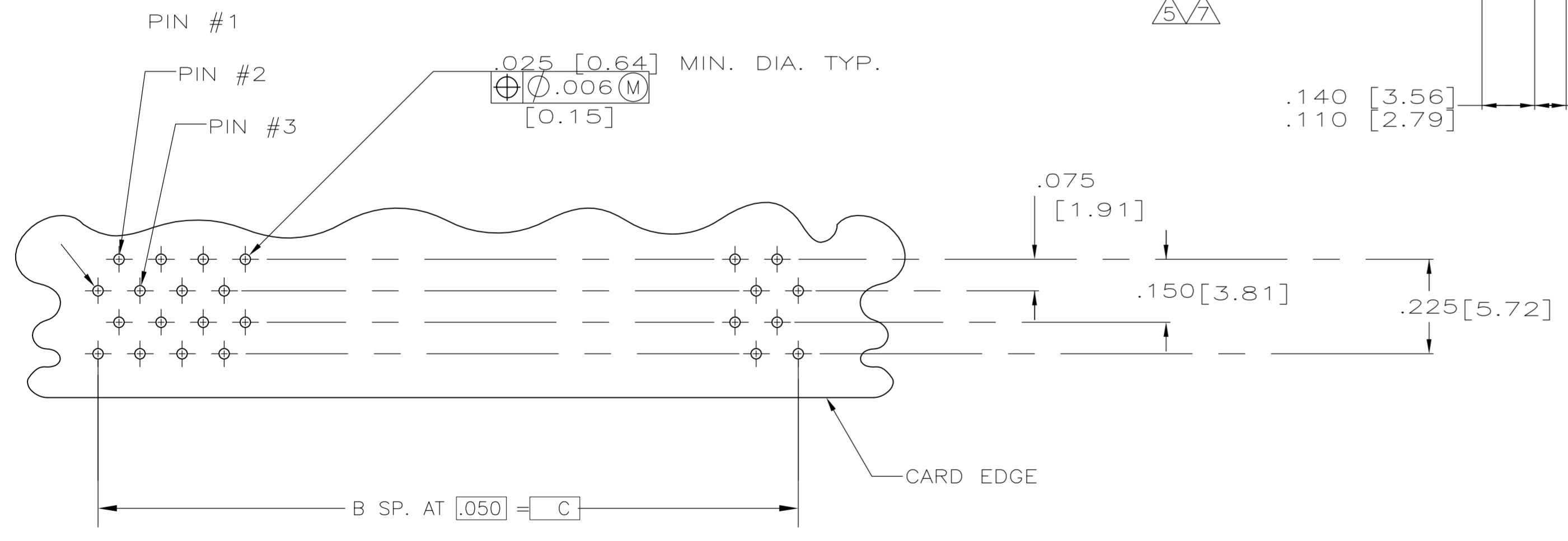
RECOMMENDED P.C. BOARD LAYOUT (CONNECTOR SIDE) (SCALE 4:1)
