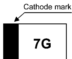
Fig. 6.1 Marking
