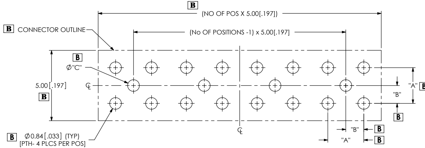
FIG 1 FOOTPRINT FOR GRFX-P-P-04-XX-ST-TH1 POSITION SHOWN
