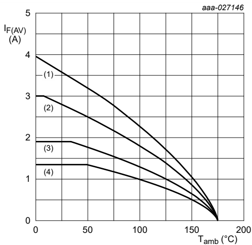
FR4 PCB, mounting pad for cathode 1 cm 2 T_j = 175\text{ }^\circ\text{C} (1) \delta = 1 ; DC (2) \delta = 0.5 ; f = 20 kHz (3) \delta = 0.2 ; f = 20 kHz (4) \delta = 0.1 ; f = 20 kHz
