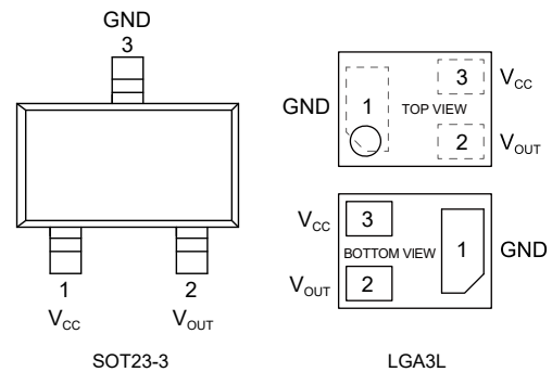
Figure 4. Pin configuration
