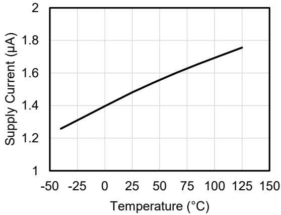
Figure 12. Supply current versus temperature ( V_{CC} = 3\text{ V} )
