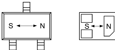
Figure 2. Sensing direction
