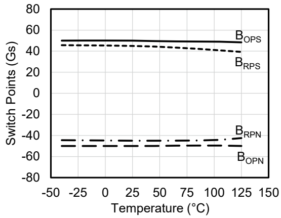
Figure 17. Switch points versus temperature ( V_{CC} = 3\text{ V} )
