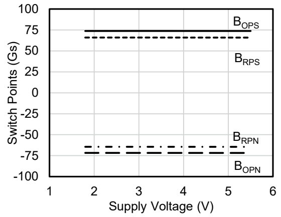
Figure 11. Switch points versus supply voltage ( T_A=25^\circ\text{C} )
