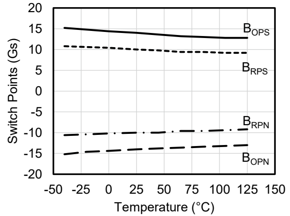
Figure 13. Switch points versus temperature ( V_{CC} = 3\text{ V} )
