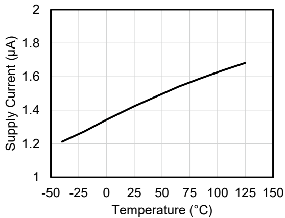
Figure 14. Supply current versus temperature ( V_{CC} = 3\text{ V} )
