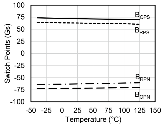
Figure 18. Switch points versus temperature ( V_{CC} = 3\text{ V} )
