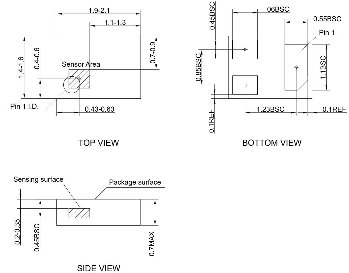
Figure 22. Package outline of LGA3L (unit: mm)
