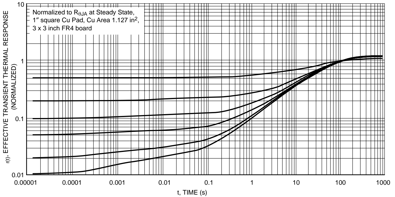
Figure 13. Thermal Response
