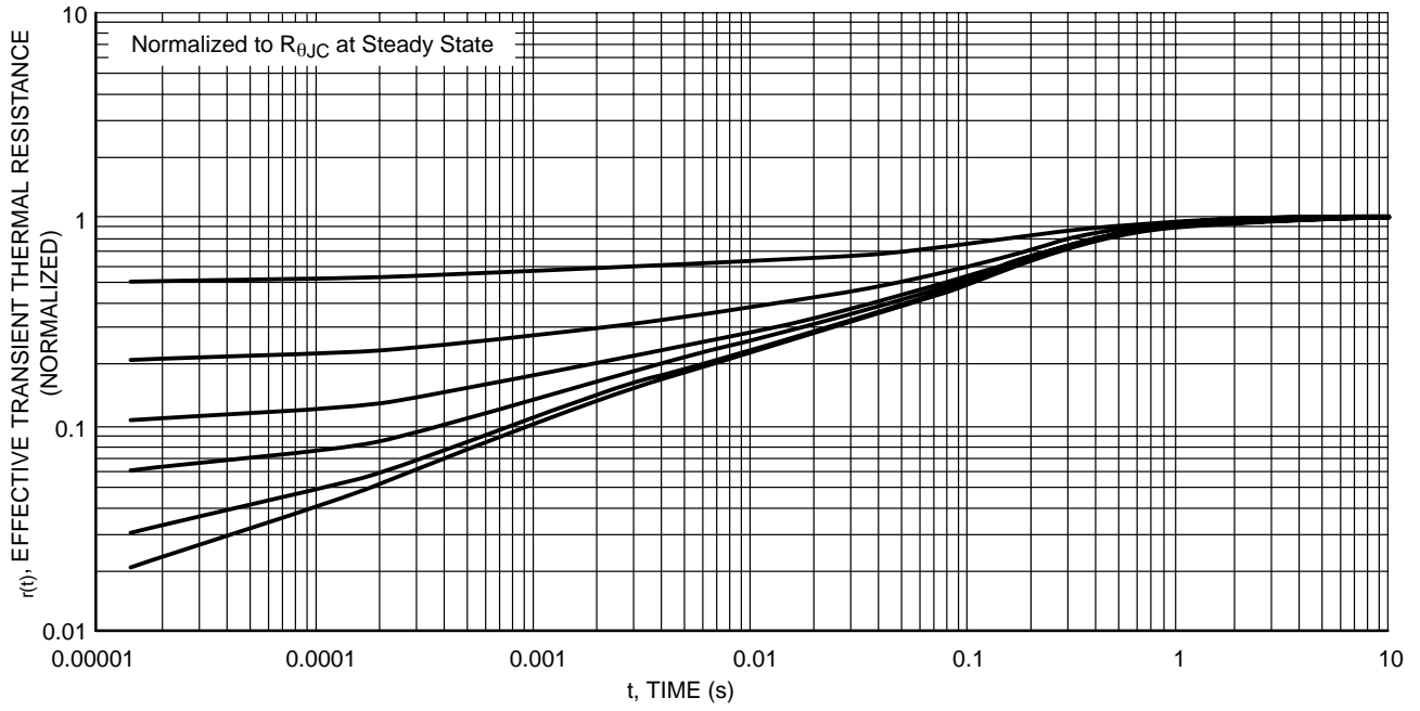
Figure 12. Thermal Response
