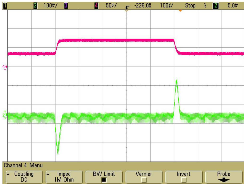
Figure 5. Transient Response Waveform at 18Vin and 3.3 – 6.7Aout (5A, 100mV, 100us / div)
