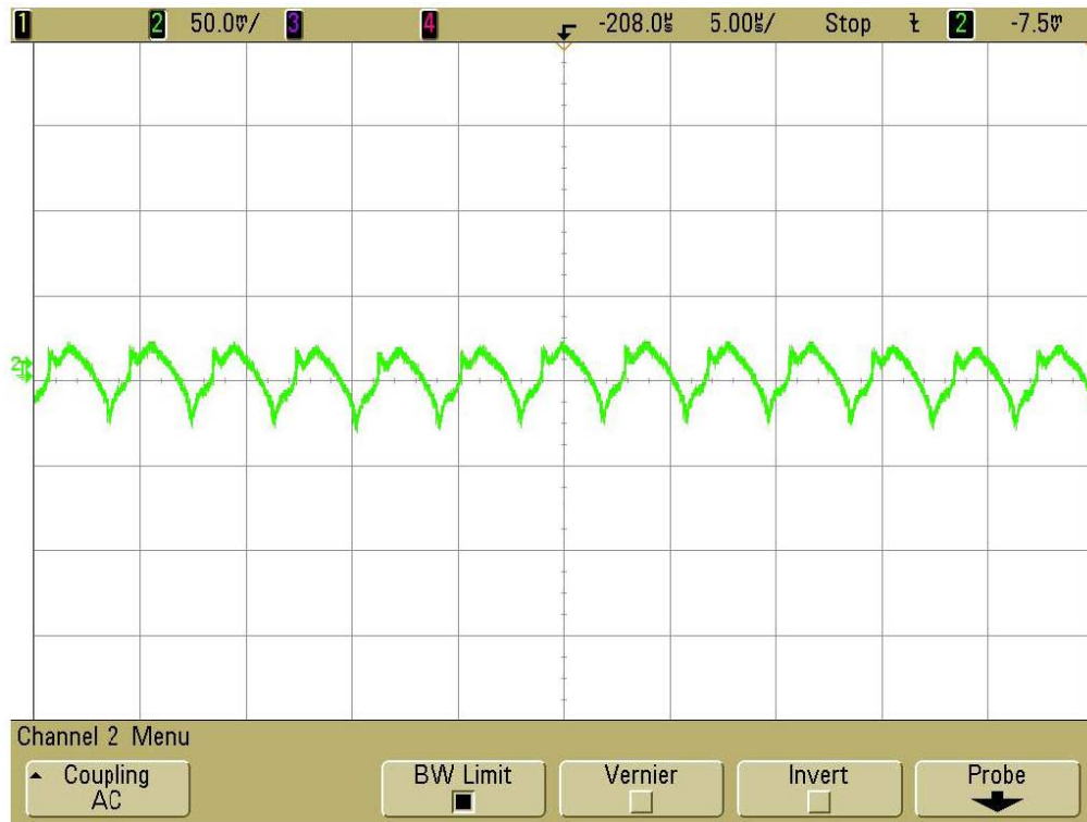
Figure 4. Output Ripple at 18Vin and 6.7Aout (50mV, 5us / div, 25MHz)
