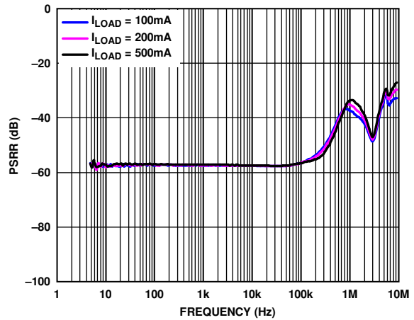
Figure 38. Power Supply Rejection Ratio (PSRR) vs. Frequency, 500 mV Headroom, V_{OUT} = 5 V
