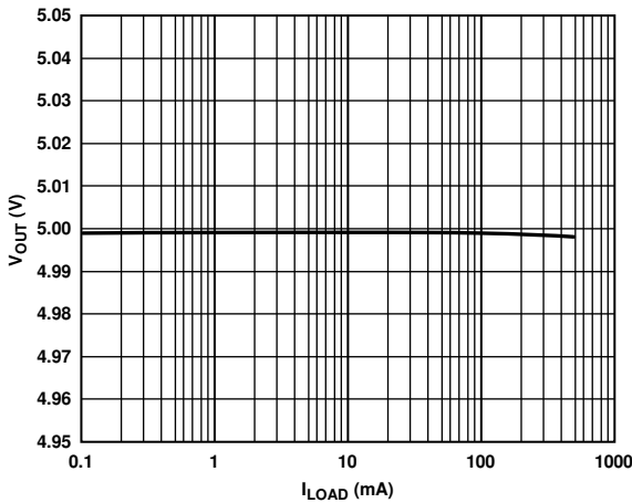
Figure 5. Output Voltage ( V_{OUT} ) vs. Load Current ( I_{LOAD} )
