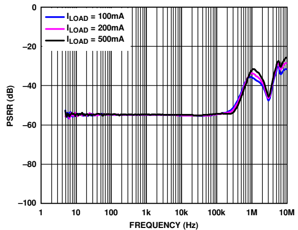
Figure 39. Power Supply Rejection Ratio (PSRR) vs. Frequency, 400 mV Headroom, V_{OUT} = 5 V
