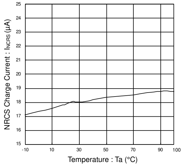
Figure 32. NRCS Charge Current vs Temperature
