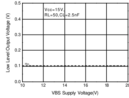
Figure 11b. Low Level Output vs VBS Supply Voltage
