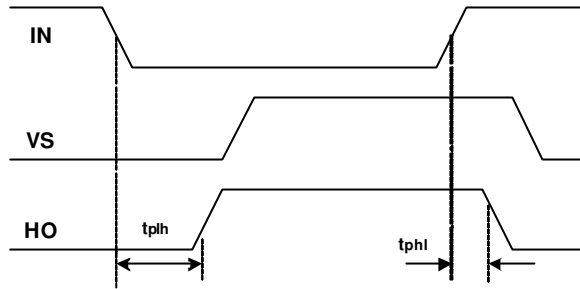
Figure 1. Input /output Timing Diagram
