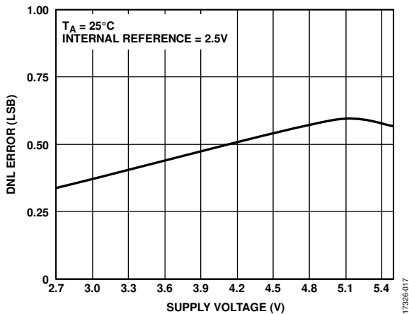
Figure 21. AD5679/AD5679R DNL Error vs. Supply Voltage
