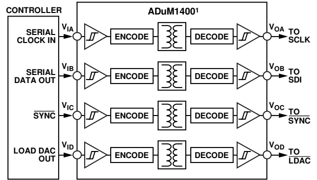
Figure 71. Isolated Interface
