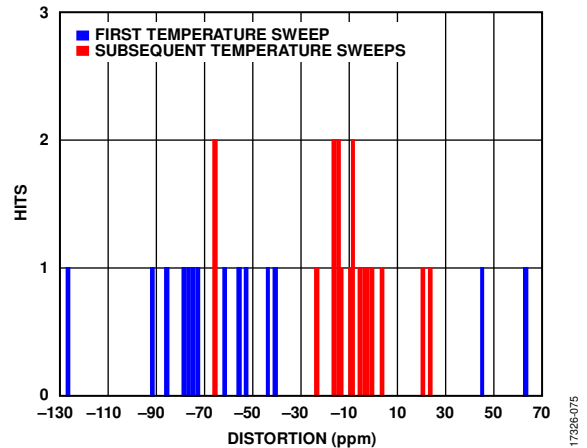
Figure 66. Thermal Hysteresis
