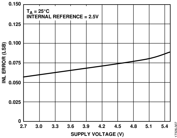
Figure 20. AD5674/AD5674R INL Error vs. Supply Voltage
