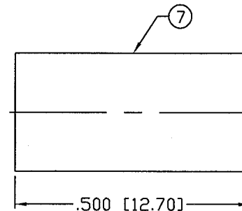
RECOMMENDED CRIMP SIZE: .213
