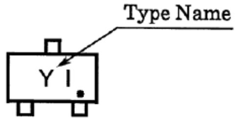
Fig. 10.2 Marking RN2108MFV
