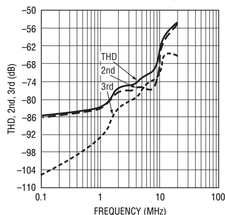
THD, 2nd, 3rd and SFDR vs Input Frequency
