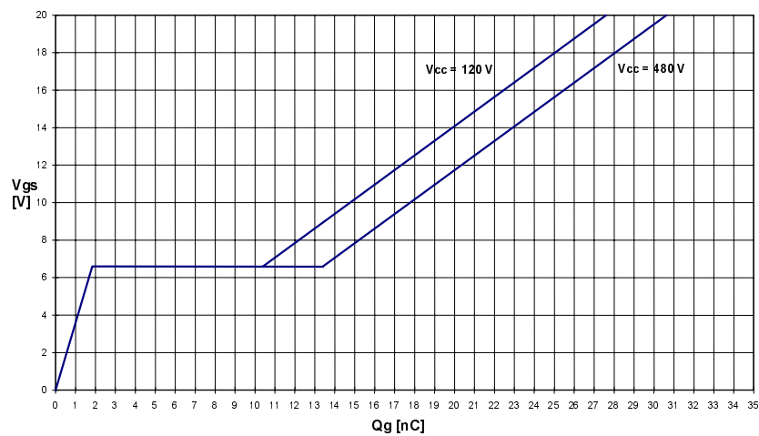
Typ. Gate-Charge
